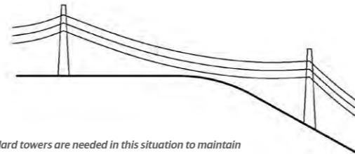
Taller than standard towers are needed in this situation to maintain clearances.
